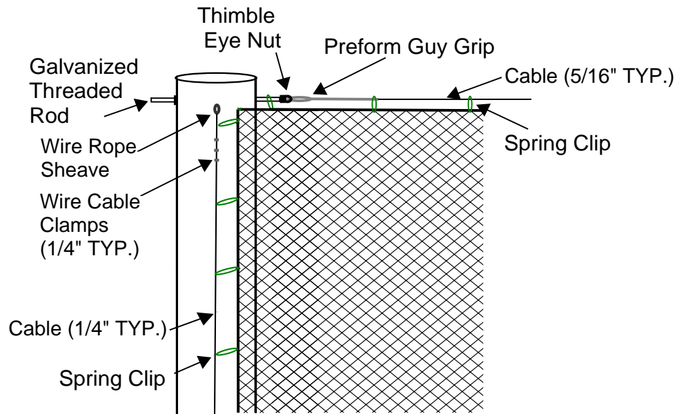
Detail A
