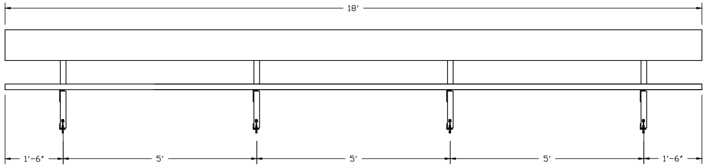
FRONT VIEW
